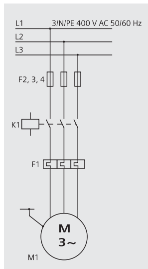
9.1.1 CIRCUITO PRINCIPAL
