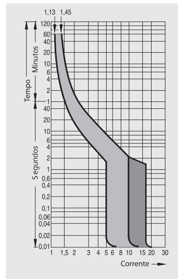
FIG 3.4 – CURVA C
